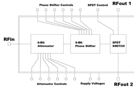
Functional Diagram
